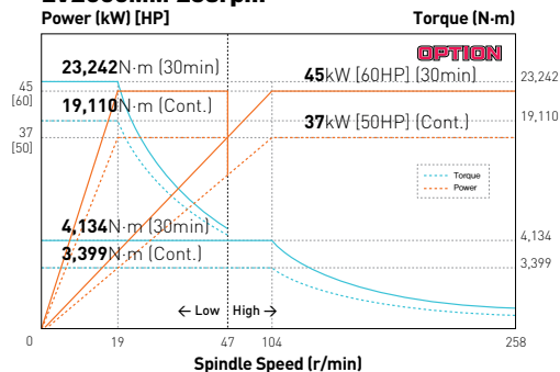
LV2000MM 258rpm
